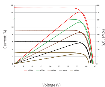
Characteristic curves (530W)
