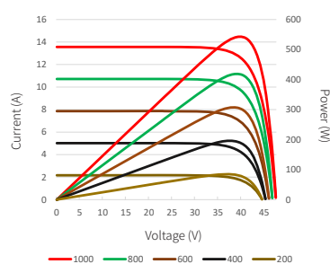
Characteristic curves (530W)
