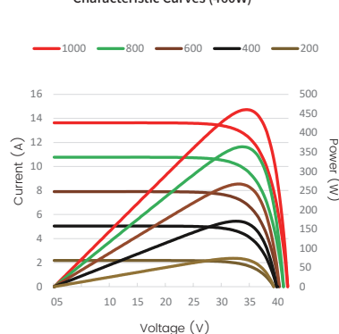
Characteristic Curves (460W)
