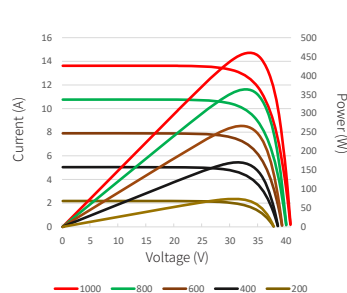
Current-Voltage & Power-Voltage Curves (465W)
